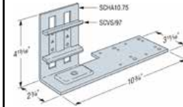
Horizontal Anchorage Slide-Clip SCHA10.75-KT
